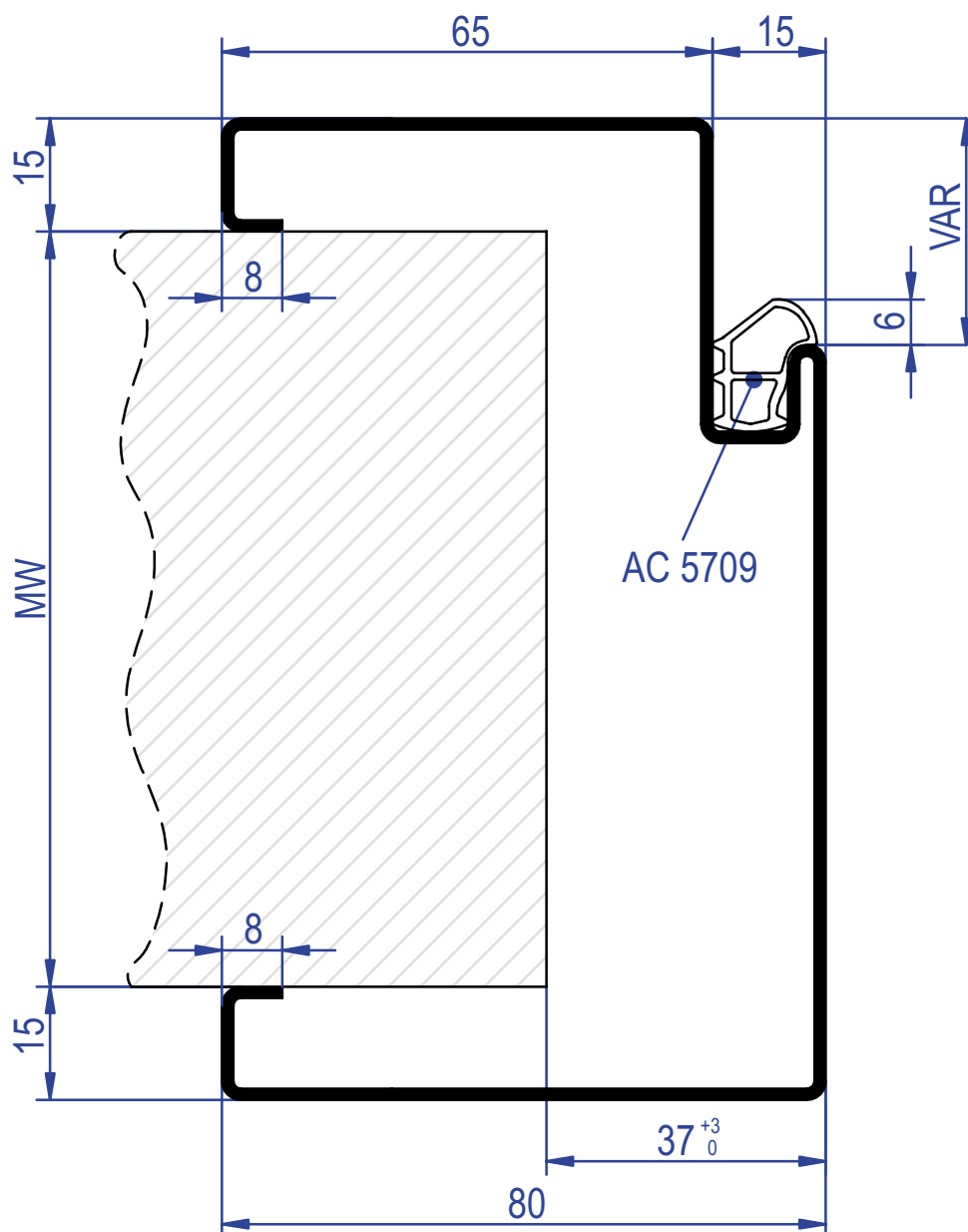
Ganzglastür porta in cristallo Glass door
