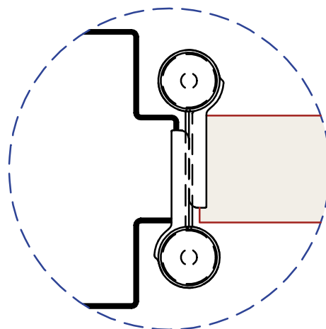
frames for double acting doors
