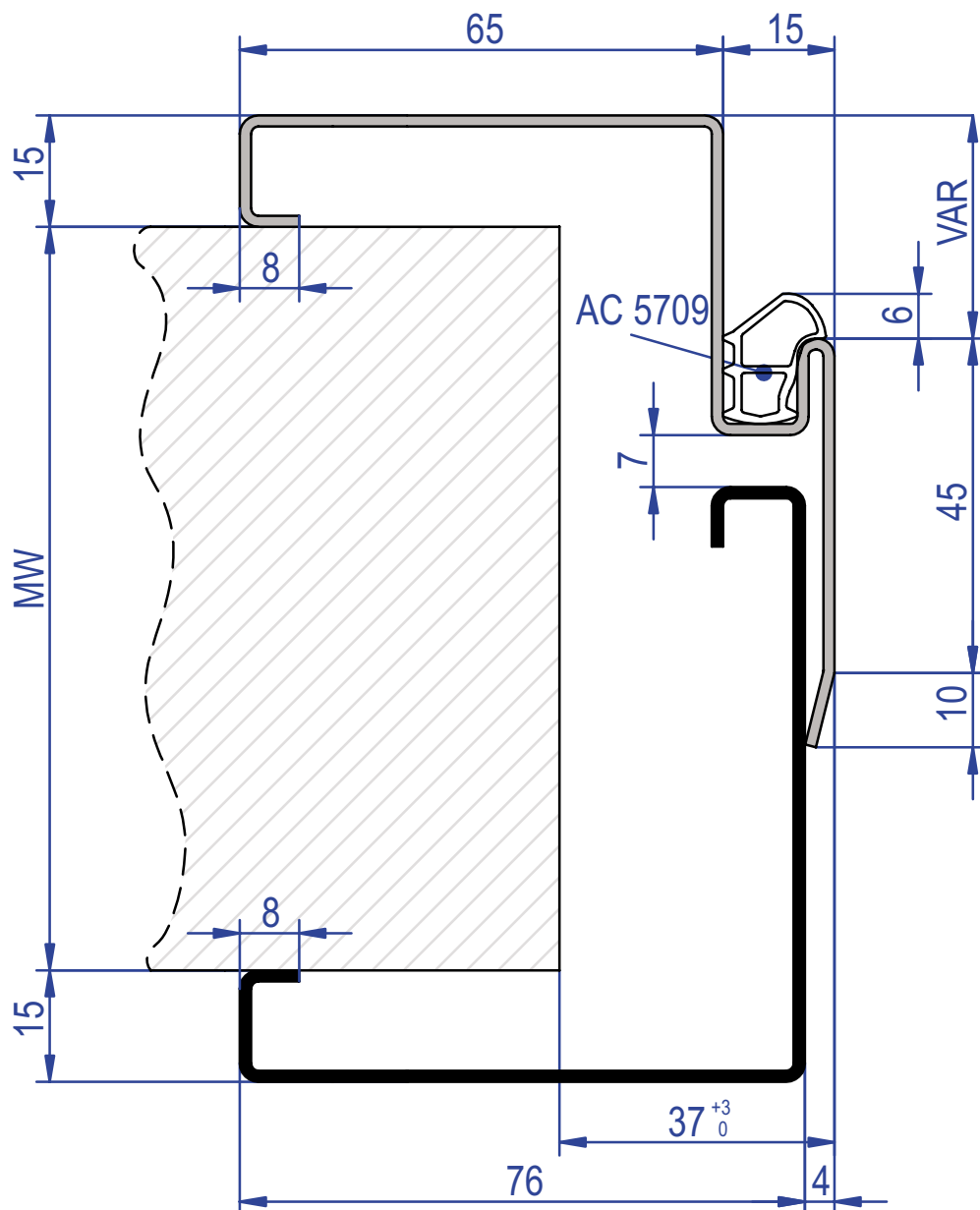
Ganzglastür porta in cristallo Glass door
