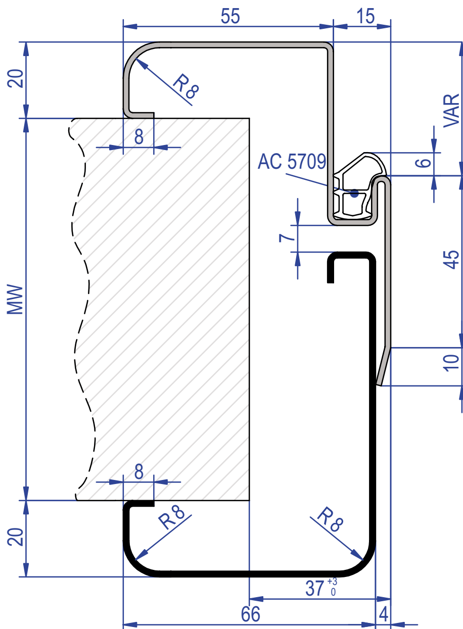
Ganzglastür porta in cristallo Glass door
