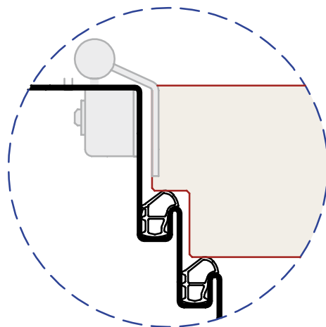
flush rebated door
