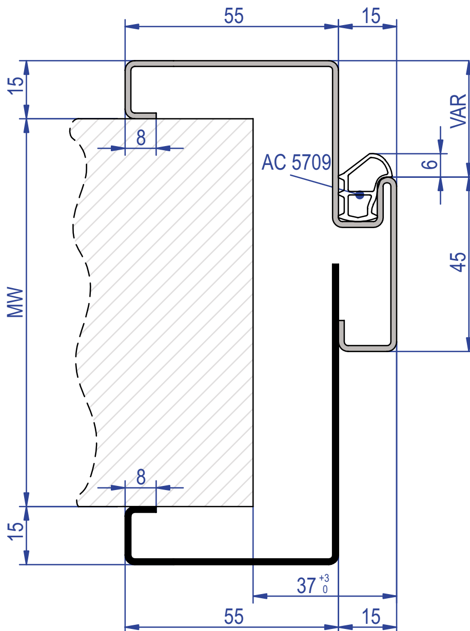
Ganzglastür porta in cristallo Glass door
