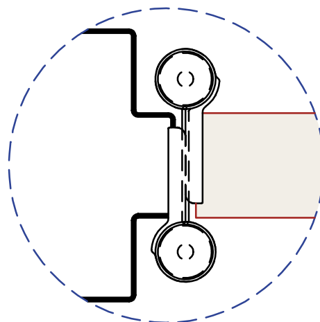
Pendeltürzargen casseporte per porta a vento frames for double acting doors
