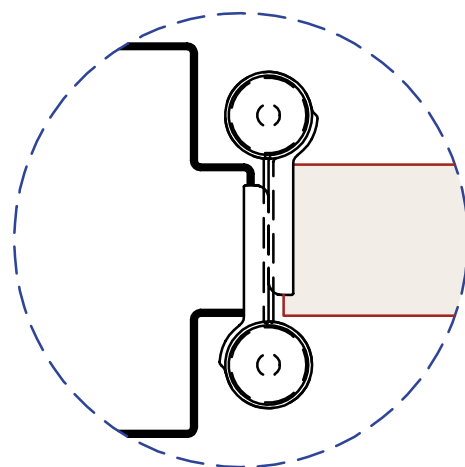
Pendeltürzargen casaporte per porta a vento frames for double acting doors
